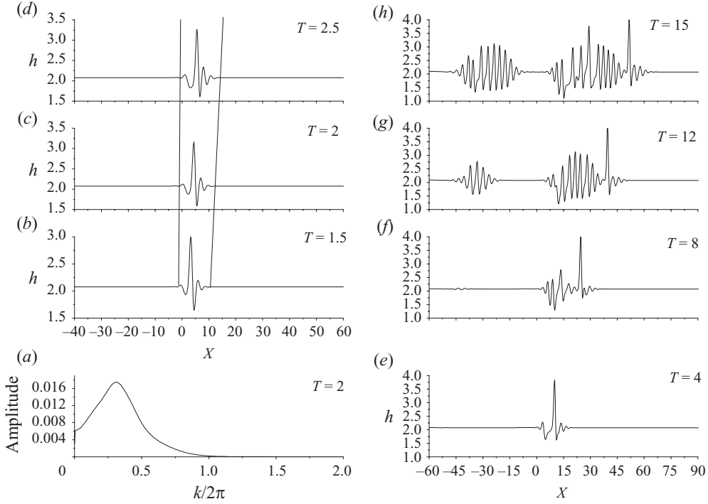
FIGURE 5. (a) Fourier transform and (b–h) snap-shots of interfacial waves for the air–deicing system in response to an impulsive disturbance; H_0 = 2.07 , \varepsilon = 0.5 , x_0 = 0.8 , We = 60 and Fr = 3.94 \times 10^4 .
